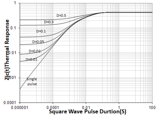
Transient Thermal Response Curve For MS65R120/TO-247
