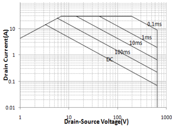
Maximum Safe Operating Area For MS65R120/TO-247
