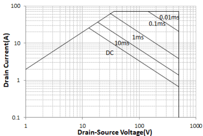
Maximum Safe Operating Area For MP18N50EI TO-220C
