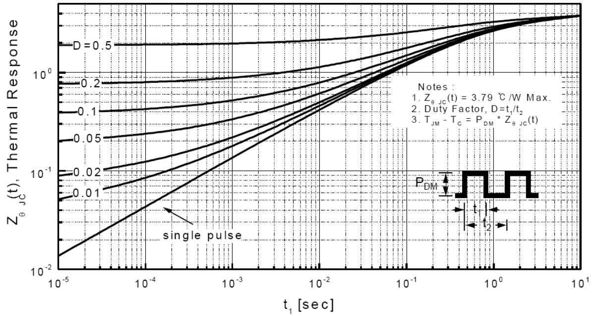
Transient Thermal Response Curve For JCS4N70FC
